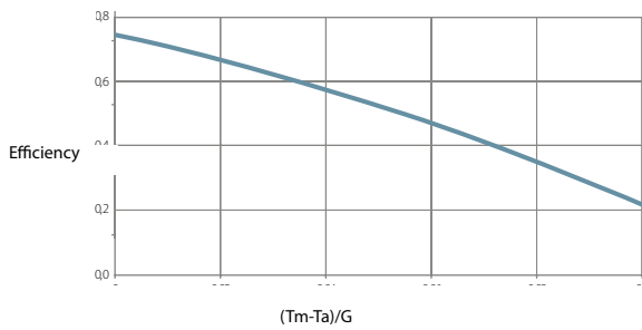
Bend of the instant efficiency
